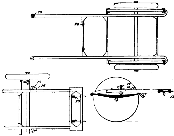
LACOÏN SEPARABLE FRAME, PLAN VIEWS AND ELEVATION.
